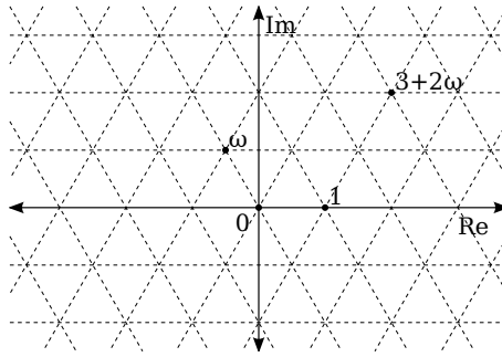
FIGURE 8.3. Eisenstein integer grid (image: Wikipedia)
