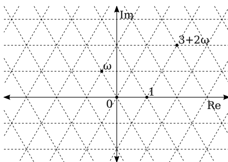
FIGURE 8.3. Eisenstein integer grid (image: Wikipedia)
